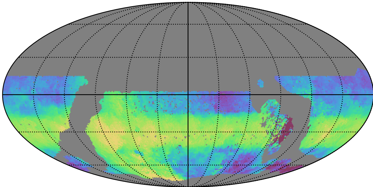
too_elab_r8_d2_giz_v3.4_10yrs WFD u band: Median HA
