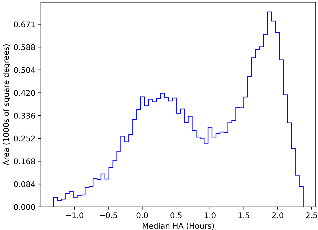
too_elab_r8_d2_giz_v3.4_10yrs WFD u band: Median HA
