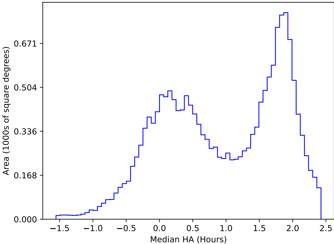
too_elab_r8_d2_giz_v3.4_10yrs WFD u band: Median HA
