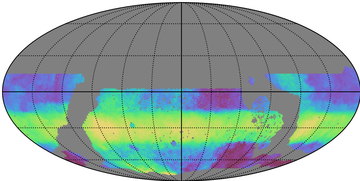
too_elab_r8_d2_giz_v3.4_10yrs WFD r band: Median HA
