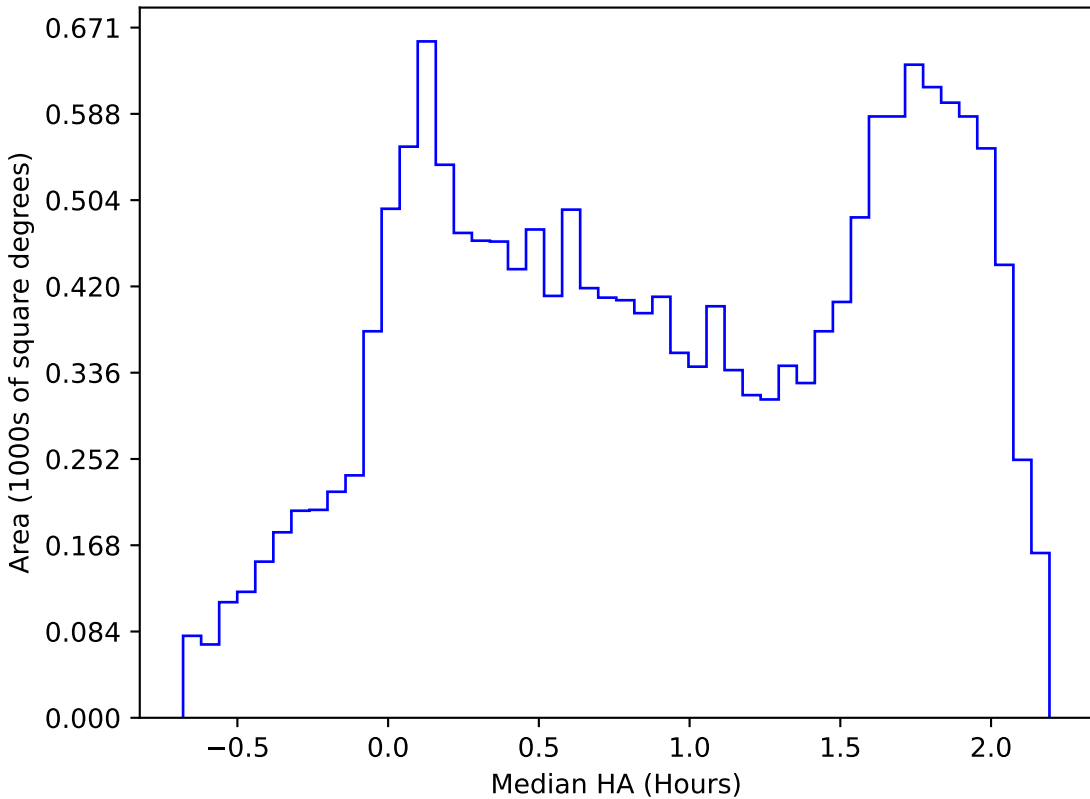
too_elab_r8_d2_giz_v3.4_10yrs WFD r band: Median HA
