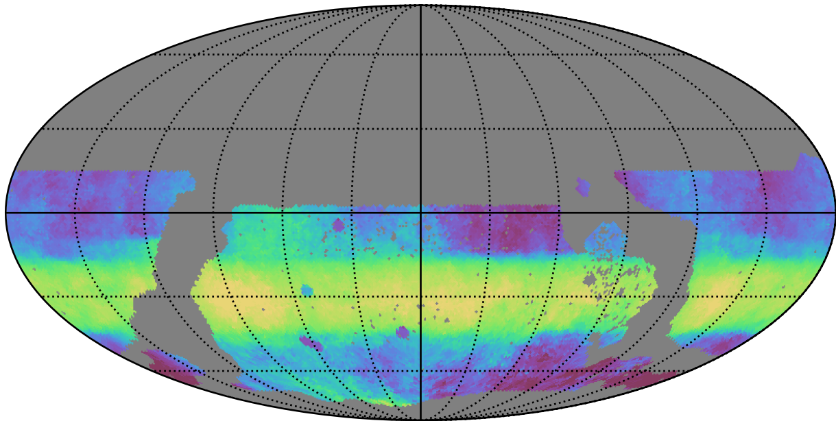
too_elab_r8_d2_giz_v3.4_10yrs WFD i band: Median HA
