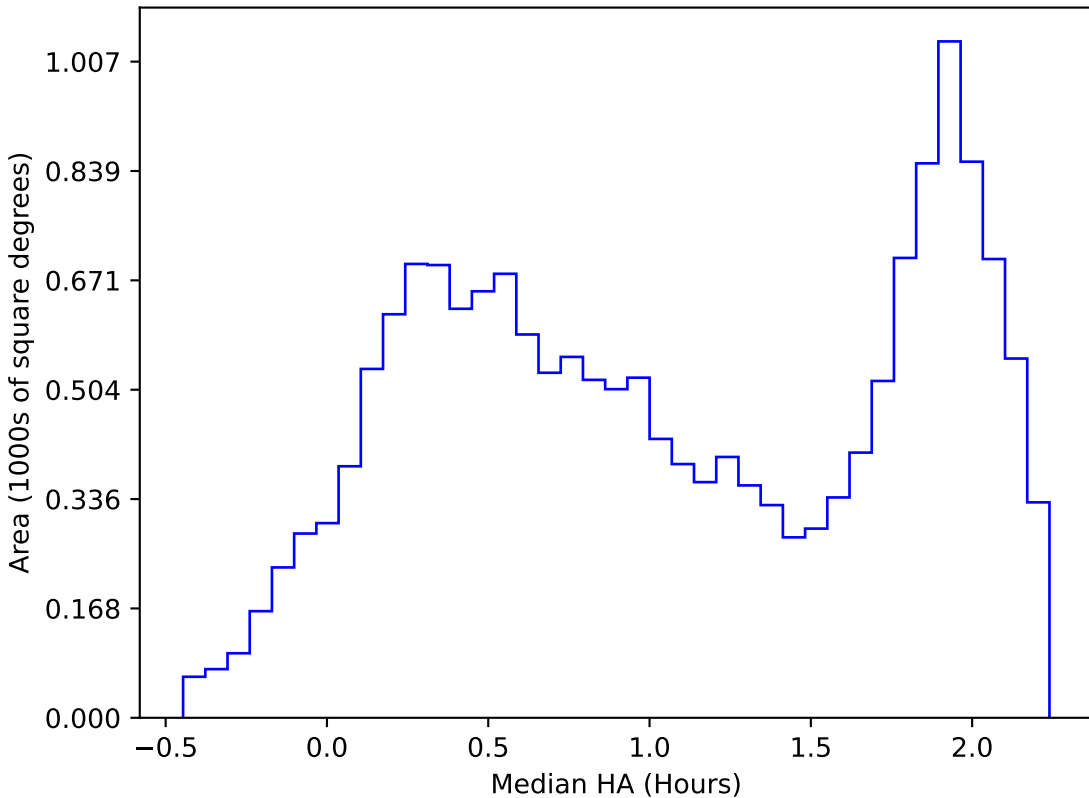
too_elab_r8_d2_giz_v3.4_10yrs WFD i band: Median HA
