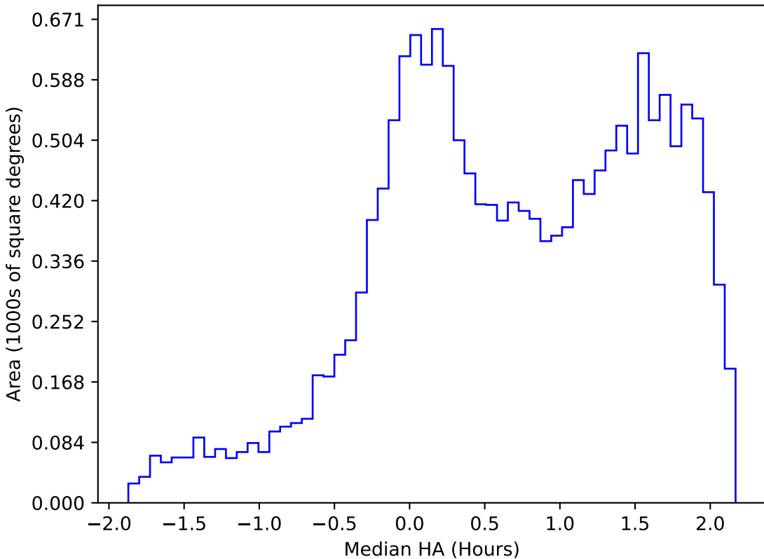
too_elab_r8_d2_giz_v3.4_10yrs WFD g band: Median HA
