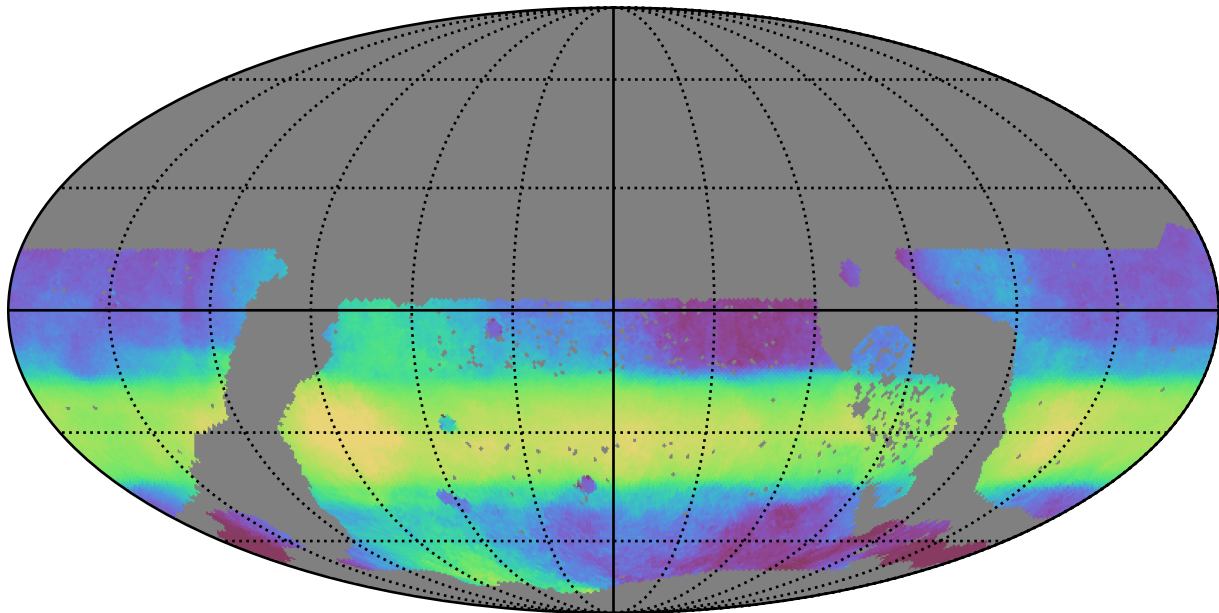
too_elab_r8_d2_giz_v3.4_10yrs WFD all bands: Median HA
