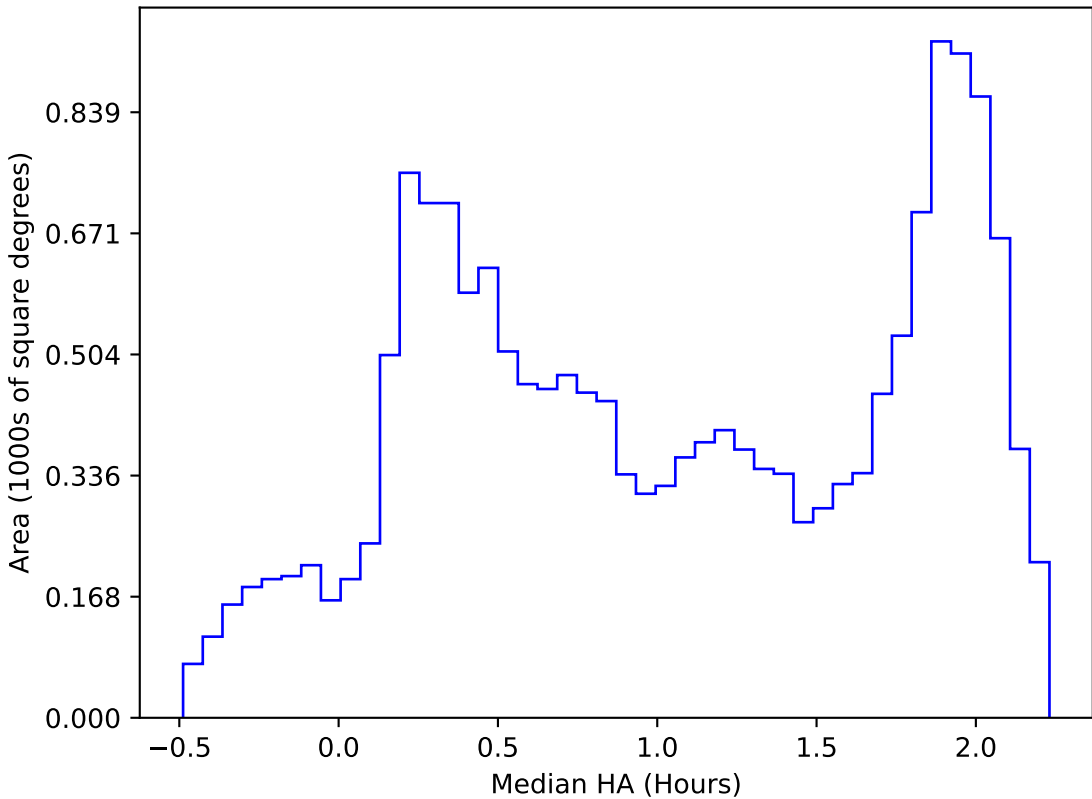
too_elab_r8_d2_giz_v3.4_10yrs WFD all bands: Median HA
