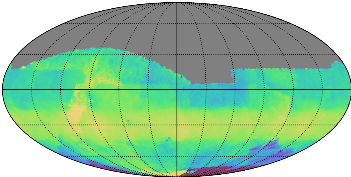
too_elab_r8_d2_giz_v3.4_10yrs All sky z band: Median HA
