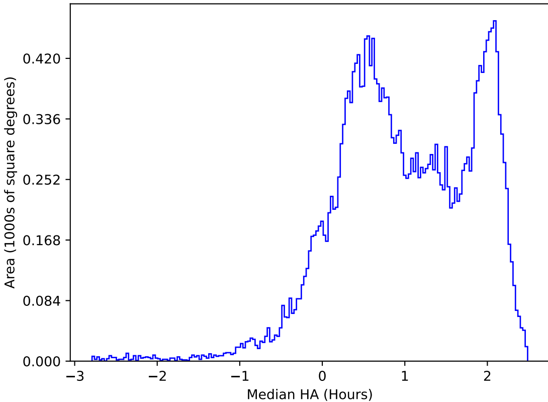
too_elab_r8_d2_giz_v3.4_10yrs All sky z band: Median HA
