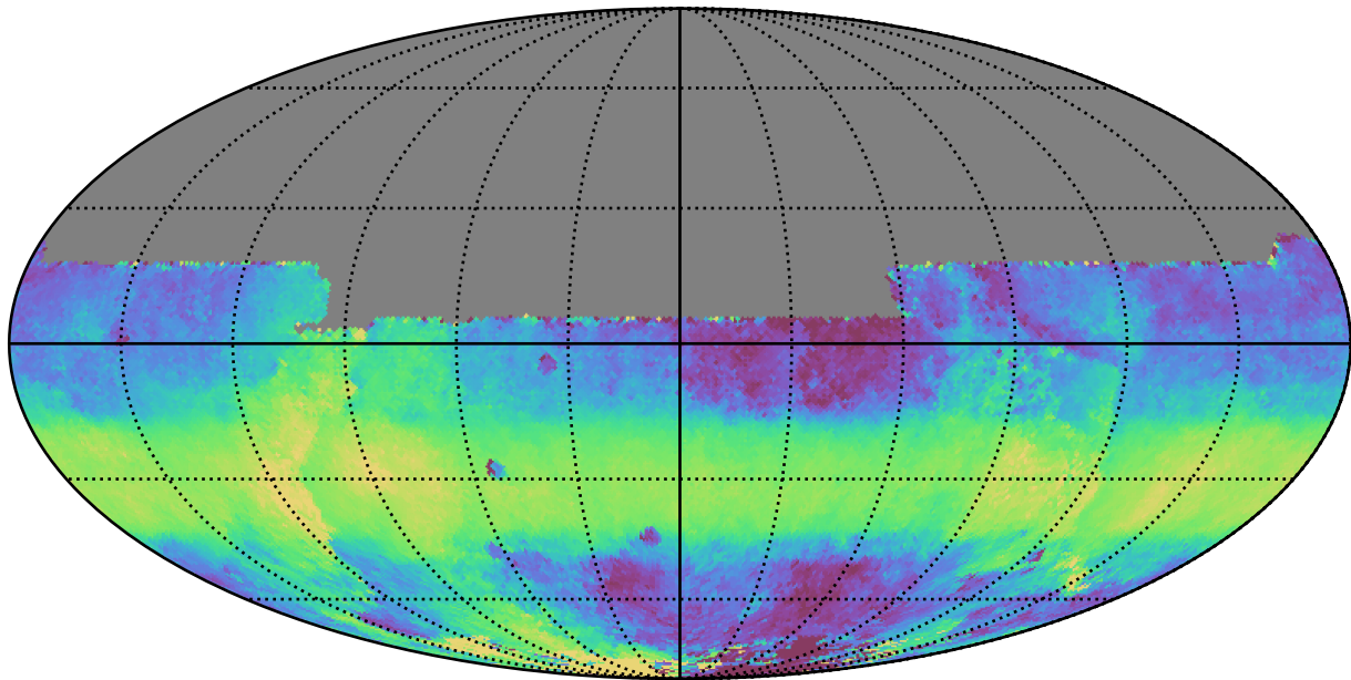
too_elab_r8_d2_giz_v3.4_10yrs All sky y band: Median HA
