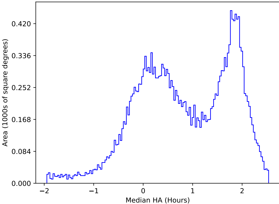
too_elab_r8_d2_giz_v3.4_10yrs All sky u band: Median HA
