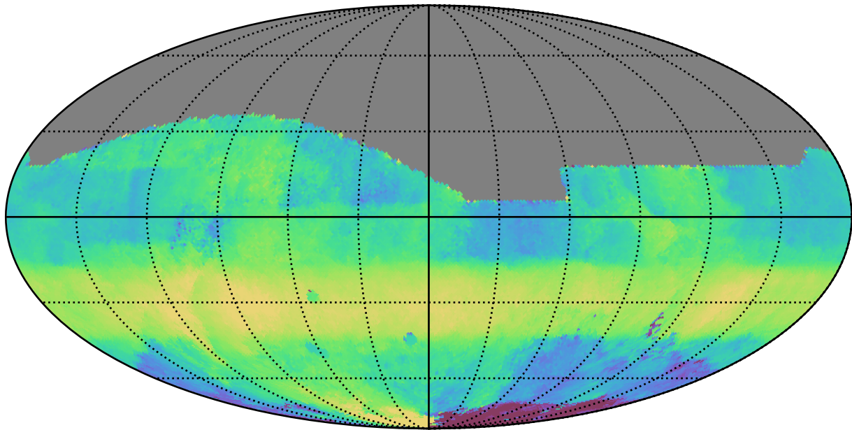
too_elab_r8_d2_giz_v3.4_10yrs All sky r band: Median HA
