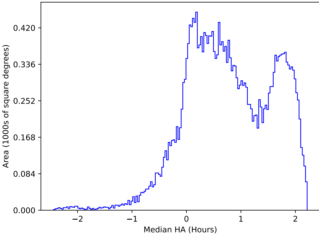
too_elab_r8_d2_giz_v3.4_10yrs All sky r band: Median HA
