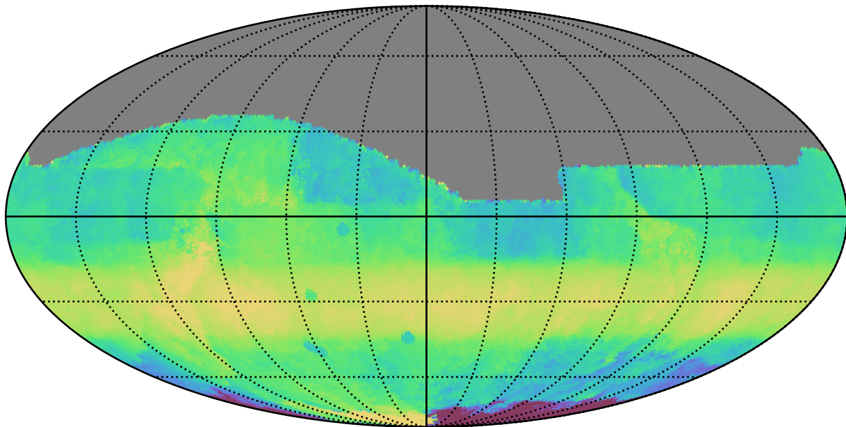
too_elab_r8_d2_giz_v3.4_10yrs All sky i band: Median HA
