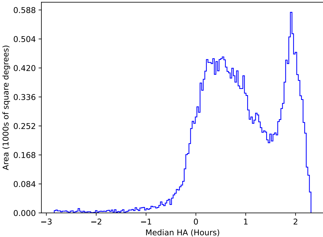
too_elab_r8_d2_giz_v3.4_10yrs All sky i band: Median HA
