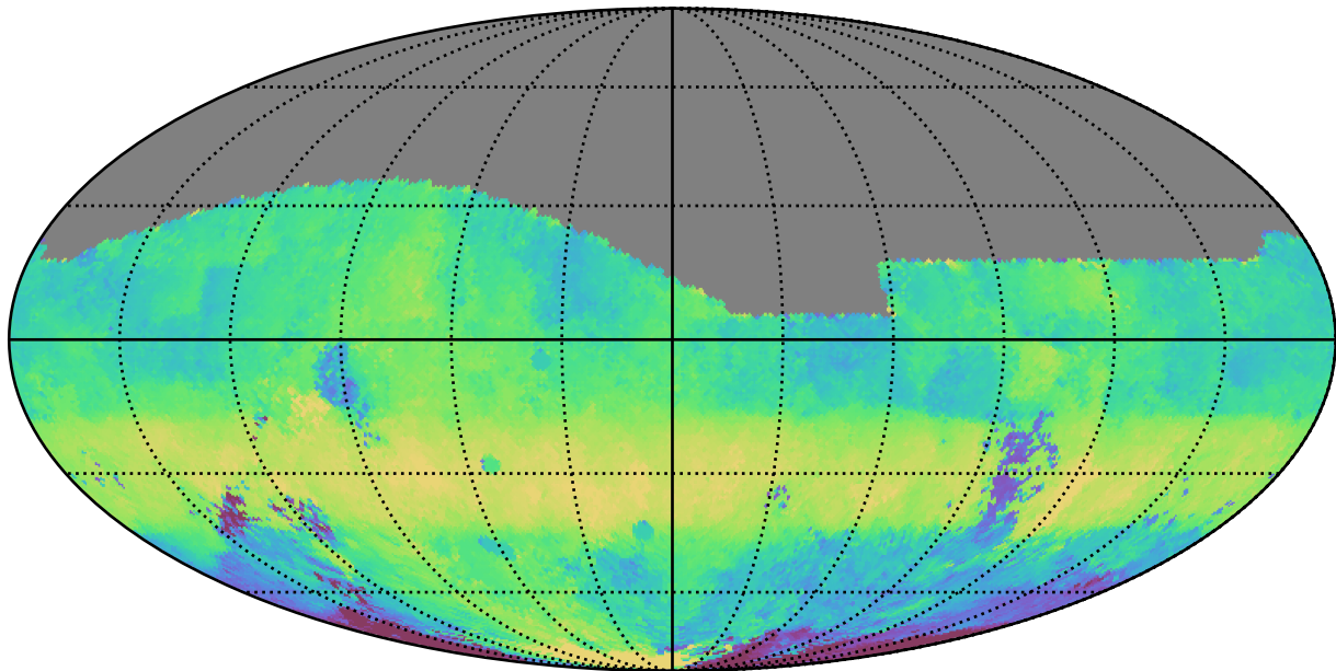
too_elab_r8_d2_giz_v3.4_10yrs All sky g band: Median HA
