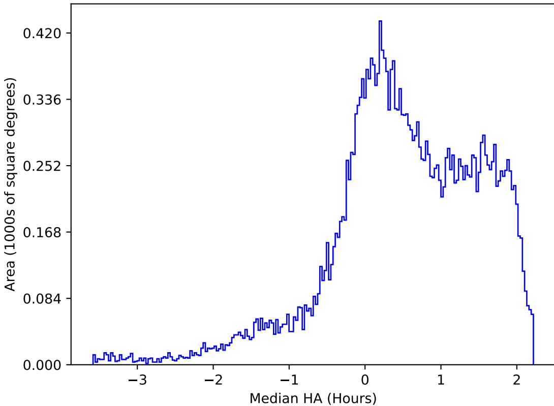
too_elab_r8_d2_giz_v3.4_10yrs All sky g band: Median HA
