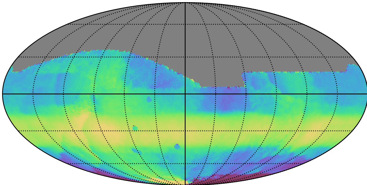
too_elab_r8_d2_giz_v3.4_10yrs All sky all bands: Median HA
