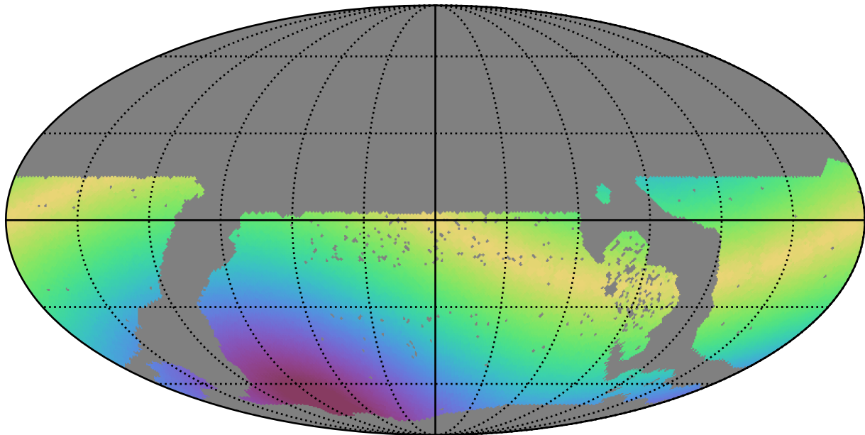
too_elab_r8_d2_giz_v3.4_10yrs WFD y band: Max solarElong
