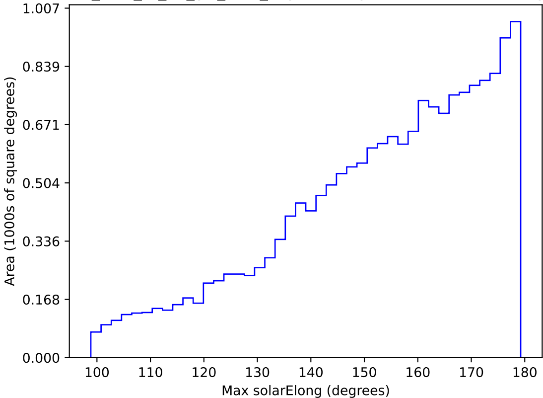
too_elab_r8_d2_giz_v3.4_10yrs WFD y band: Max solarElong
