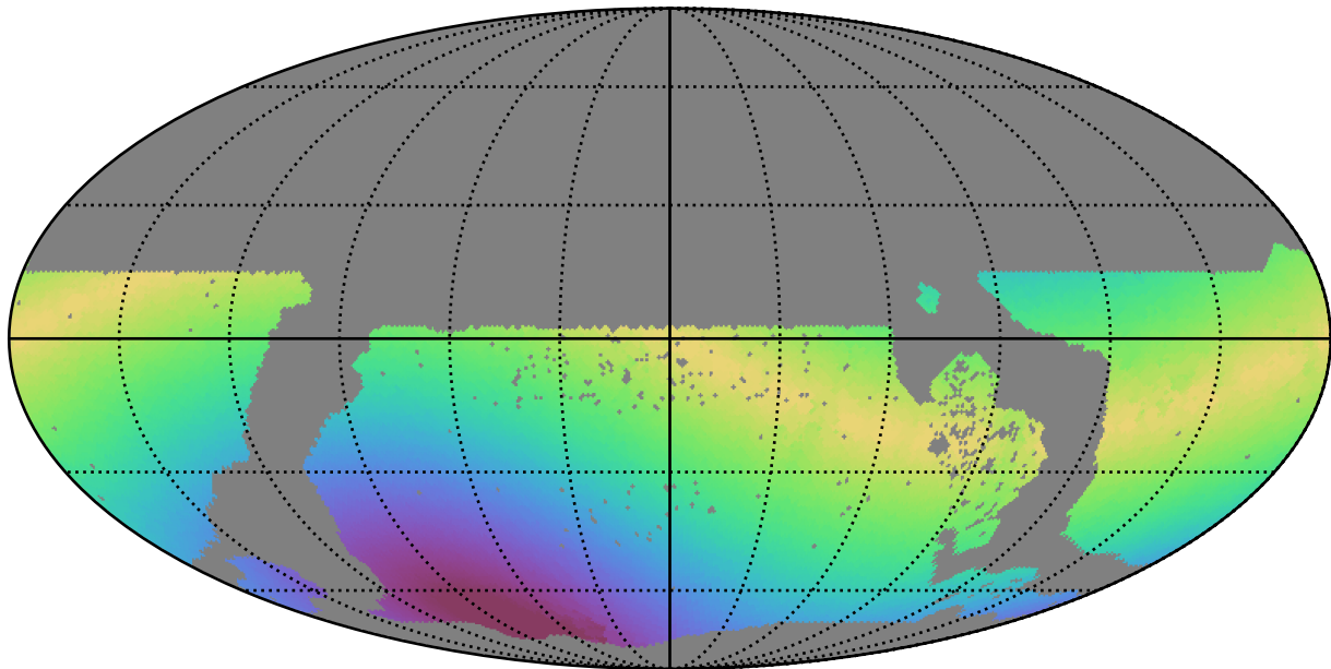
too_elab_r8_d2_giz_v3.4_10yrs WFD u band: Max solarElong
