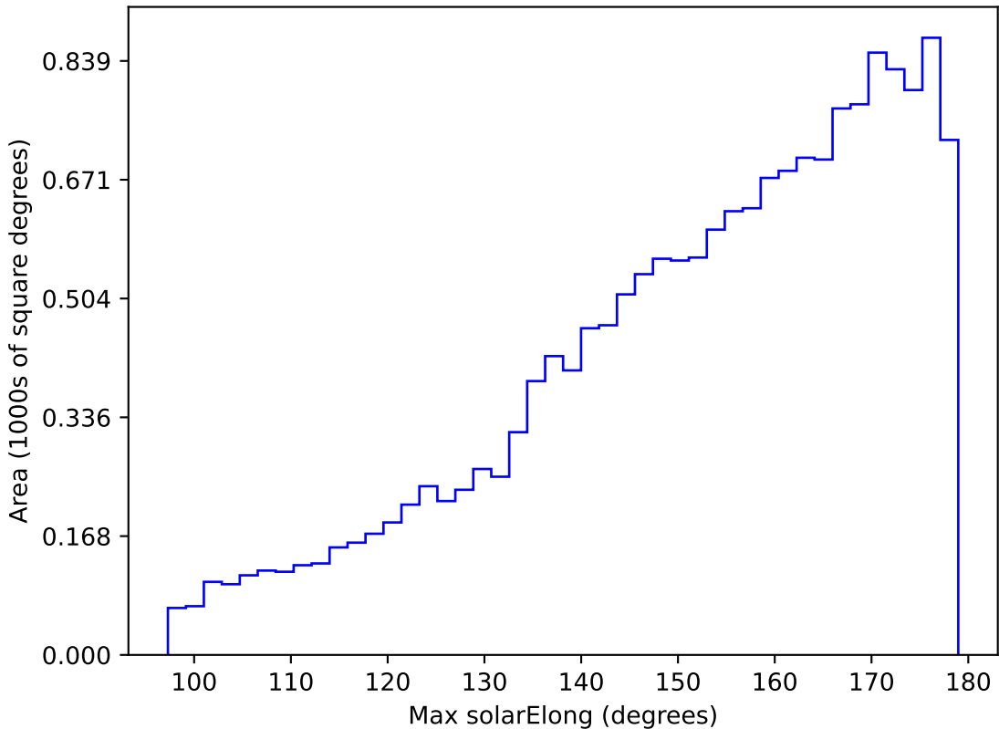
too_elab_r8_d2_giz_v3.4_10yrs WFD u band: Max solarElong
