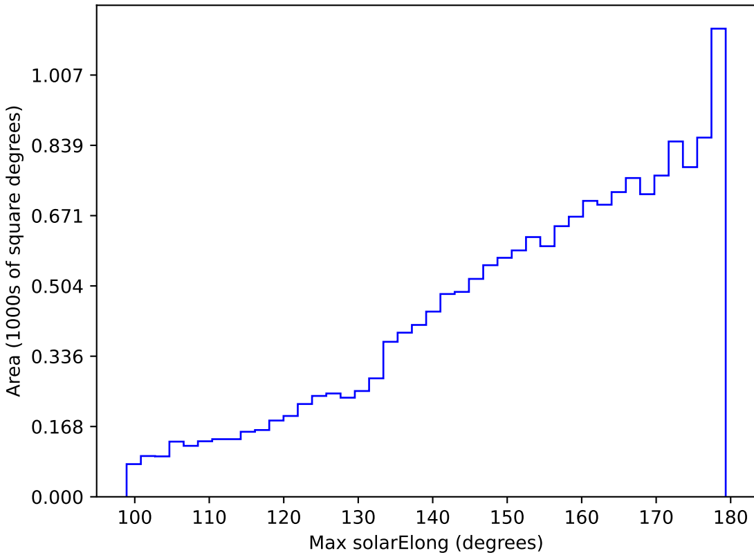
too_elab_r8_d2_giz_v3.4_10yrs WFD i band: Max solarElong
