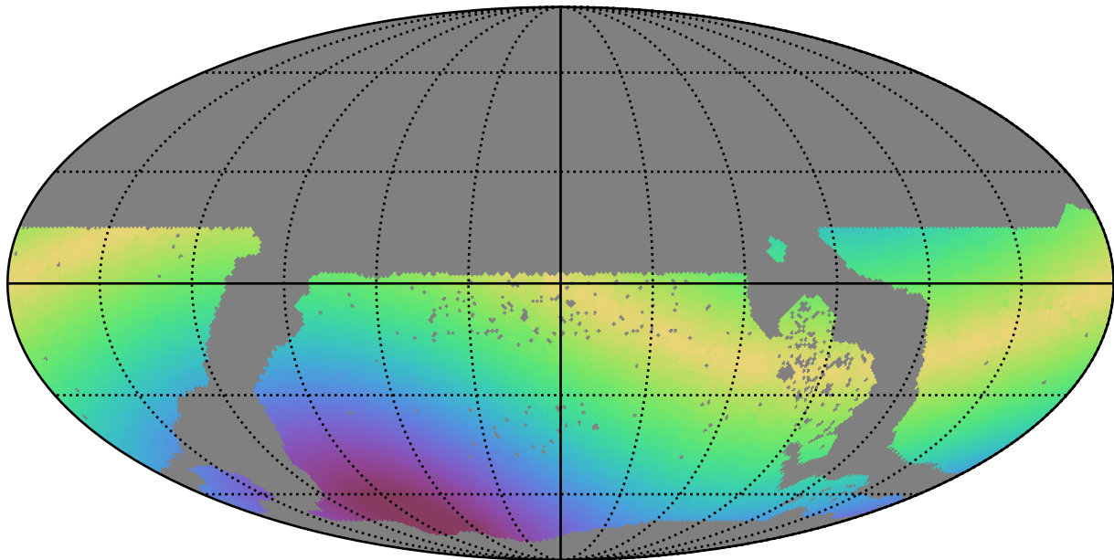
too_elab_r8_d2_giz_v3.4_10yrs WFD g band: Max solarElong
