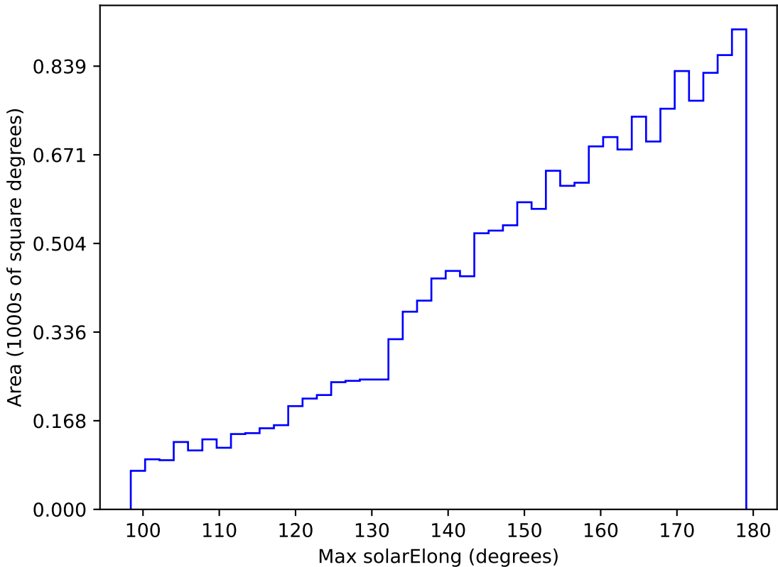
too_elab_r8_d2_giz_v3.4_10yrs WFD g band: Max solarElong
