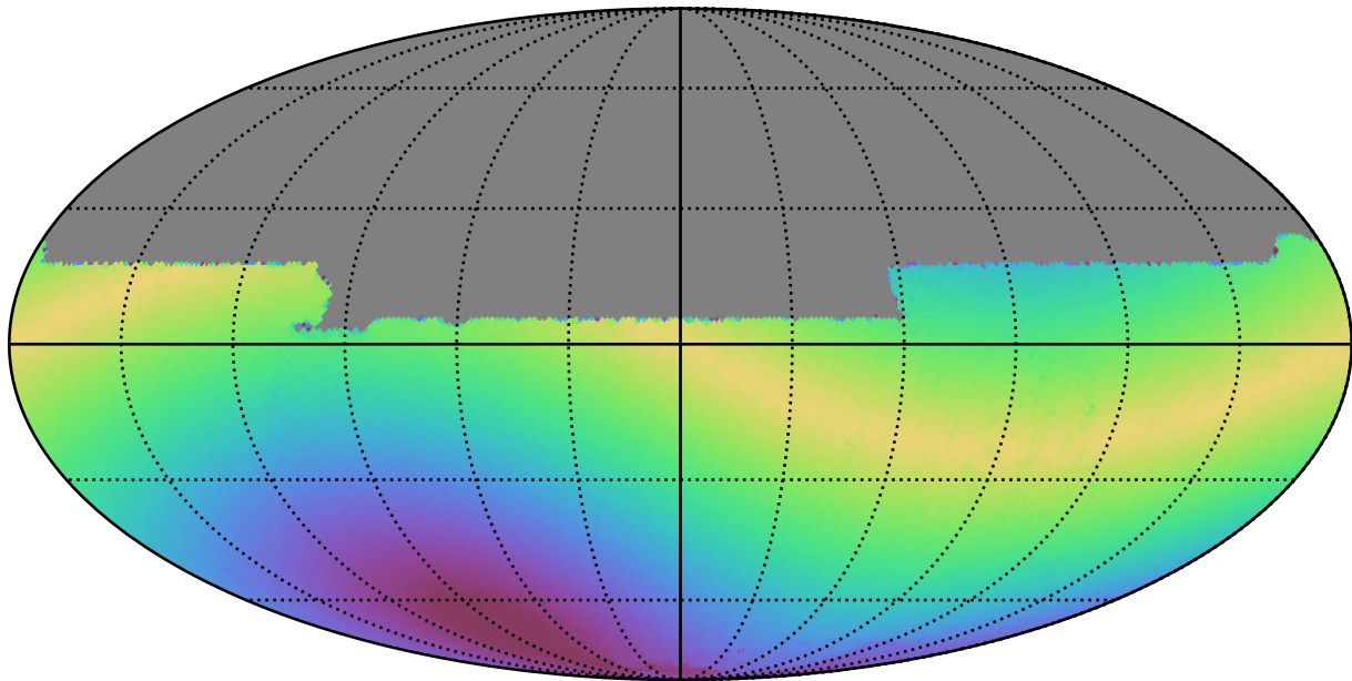
too_elab_r8_d2_giz_v3.4_10yrs All sky y band: Max solarElong
