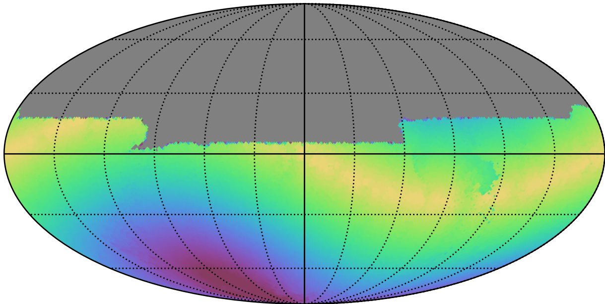
too_elab_r8_d2_giz_v3.4_10yrs All sky u band: Max solarElong
