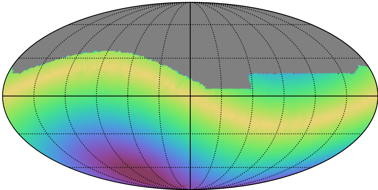
too_elab_r8_d2_giz_v3.4_10yrs All sky r band: Max solarElong
