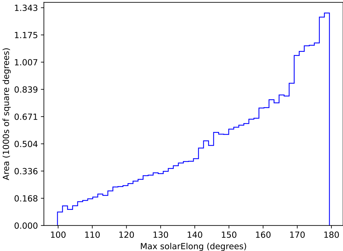
too_elab_r8_d2_giz_v3.4_10yrs All sky r band: Max solarElong
