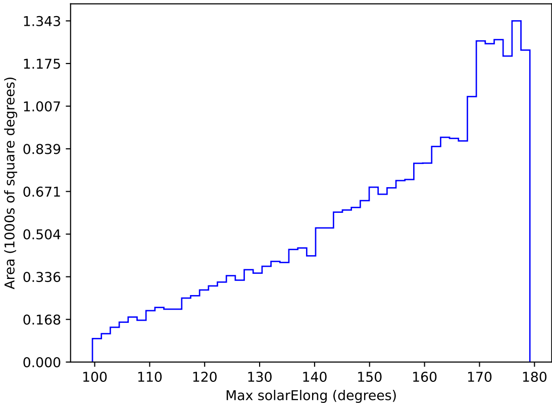
too_elab_r8_d2_giz_v3.4_10yrs All sky g band: Max solarElong
