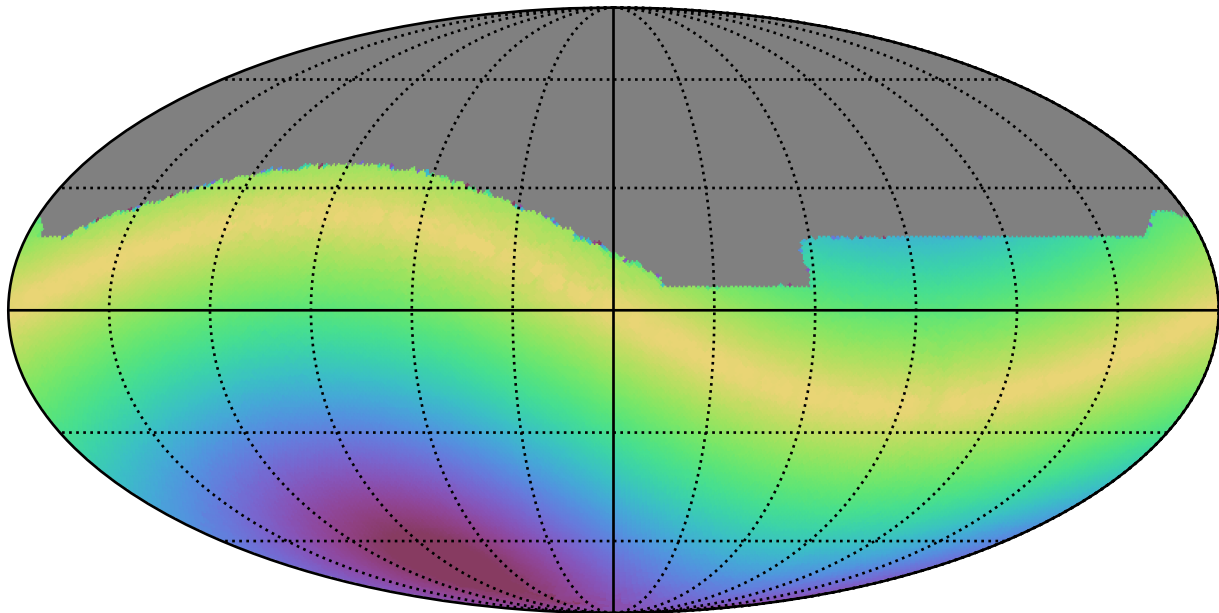
too_elab_r8_d2_giz_v3.4_10yrs All sky all bands: Max solarElong
