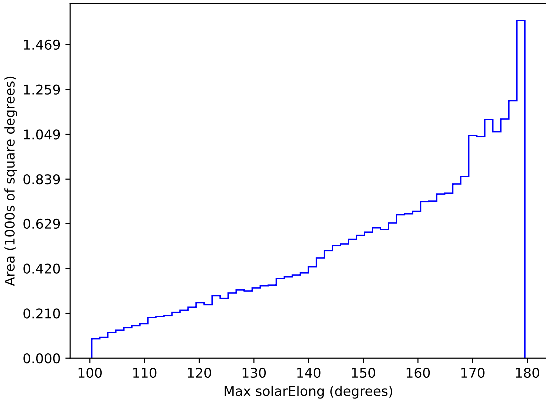
too_elab_r8_d2_giz_v3.4_10yrs All sky all bands: Max solarElong
