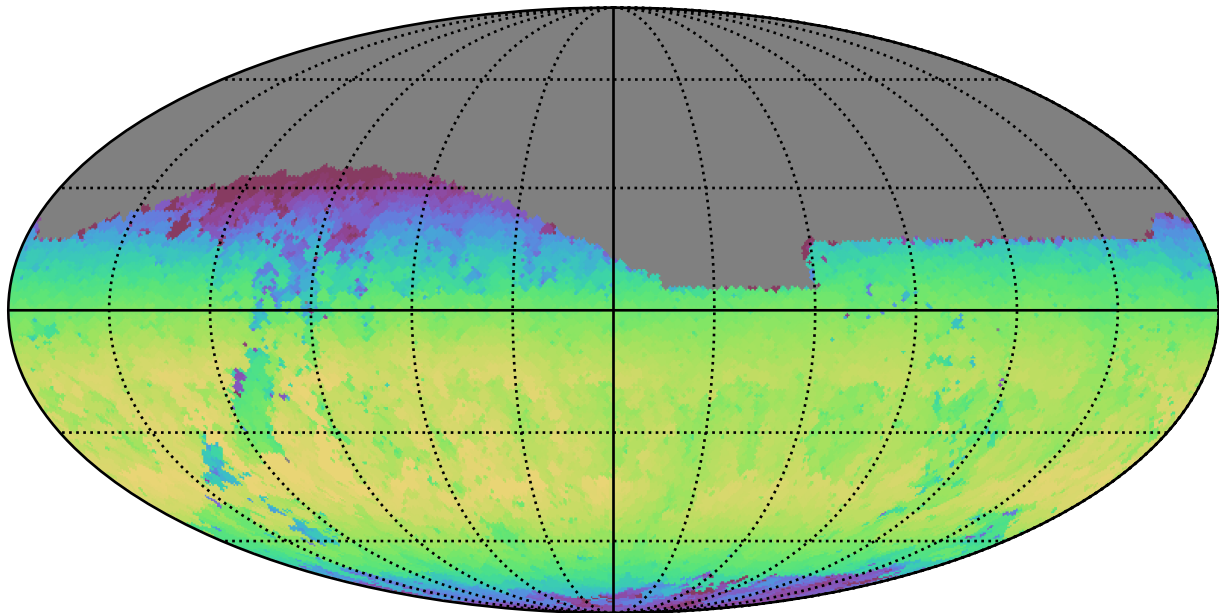
too_elab_r8_d2_giz_v3.4_10yrs Yr 1 z band: Max skyBrightness
