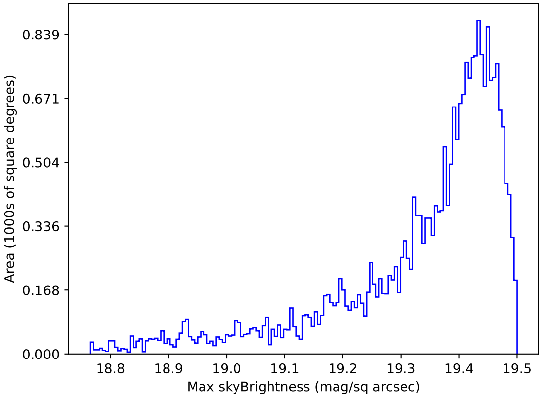
too_elab_r8_d2_giz_v3.4_10yrs Yr 1 z band: Max skyBrightness
