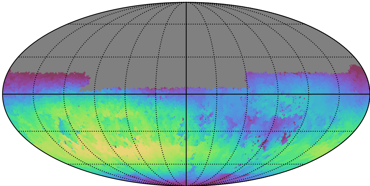
too_elab_r8_d2_giz_v3.4_10yrs Yr 1 u band: Max skyBrightness
