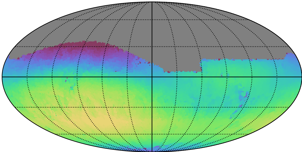
too_elab_r8_d2_giz_v3.4_10yrs Yr 1 r band: Max skyBrightness
