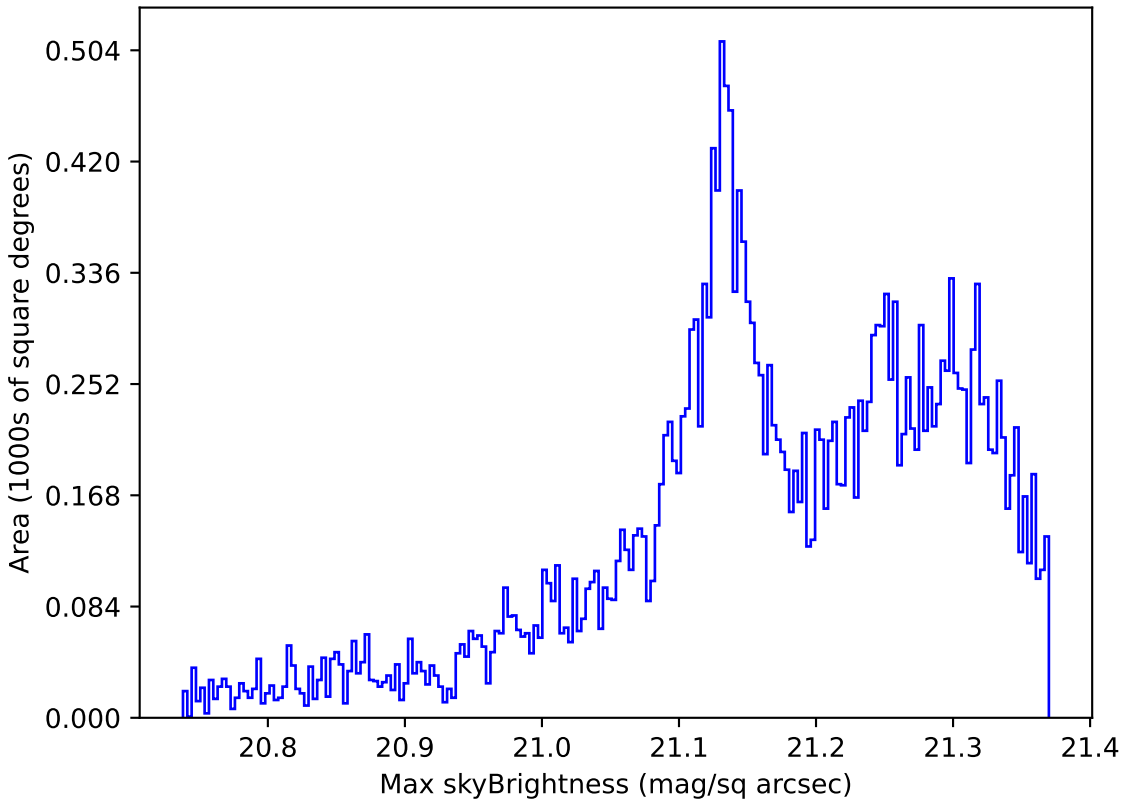
too_elab_r8_d2_giz_v3.4_10yrs Yr 1 r band: Max skyBrightness
