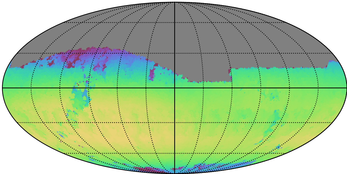
too_elab_r8_d2_giz_v3.4_10yrs Yr 1 i band: Max skyBrightness
