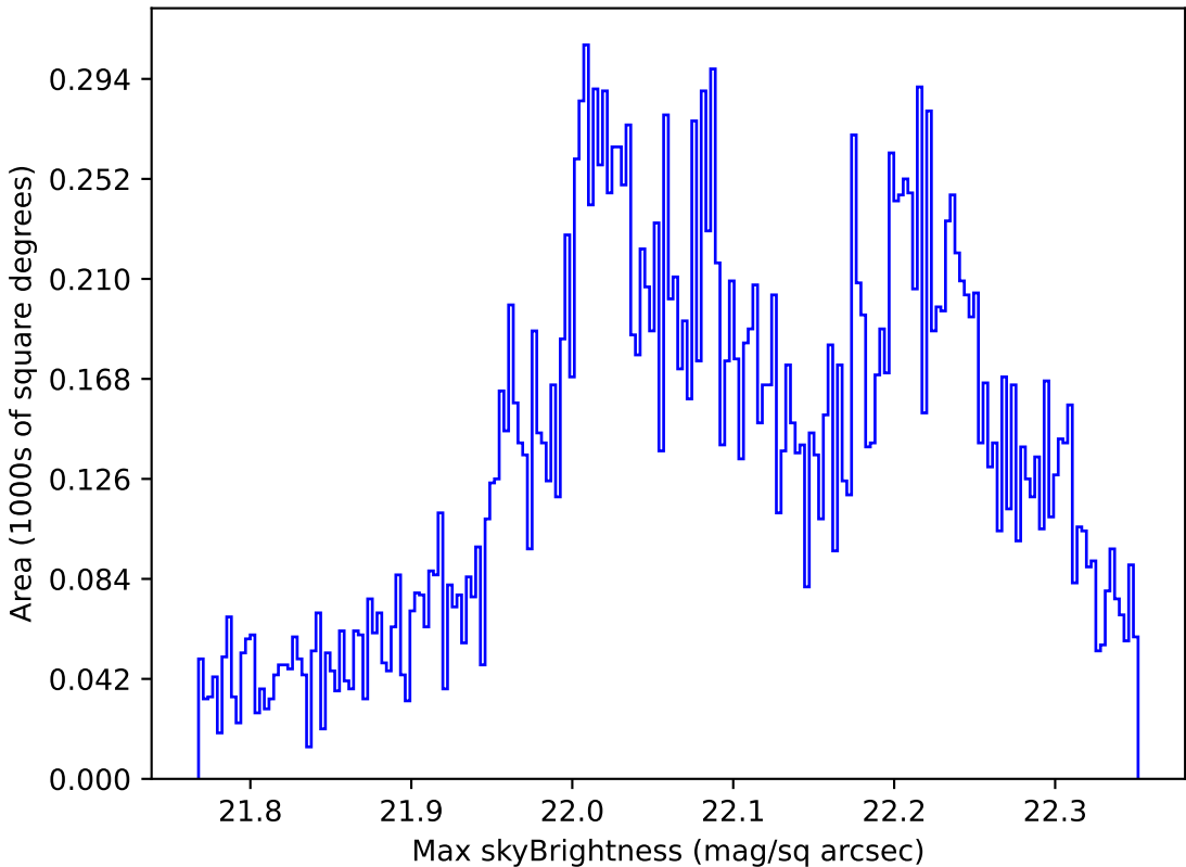
too_elab_r8_d2_giz_v3.4_10yrs Yr 1 g band: Max skyBrightness
