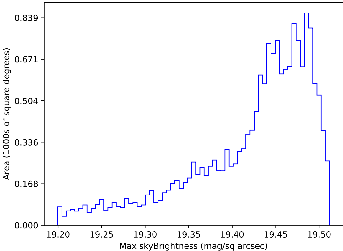
too_elab_r8_d2_giz_v3.4_10yrs WFD z band: Max skyBrightness
