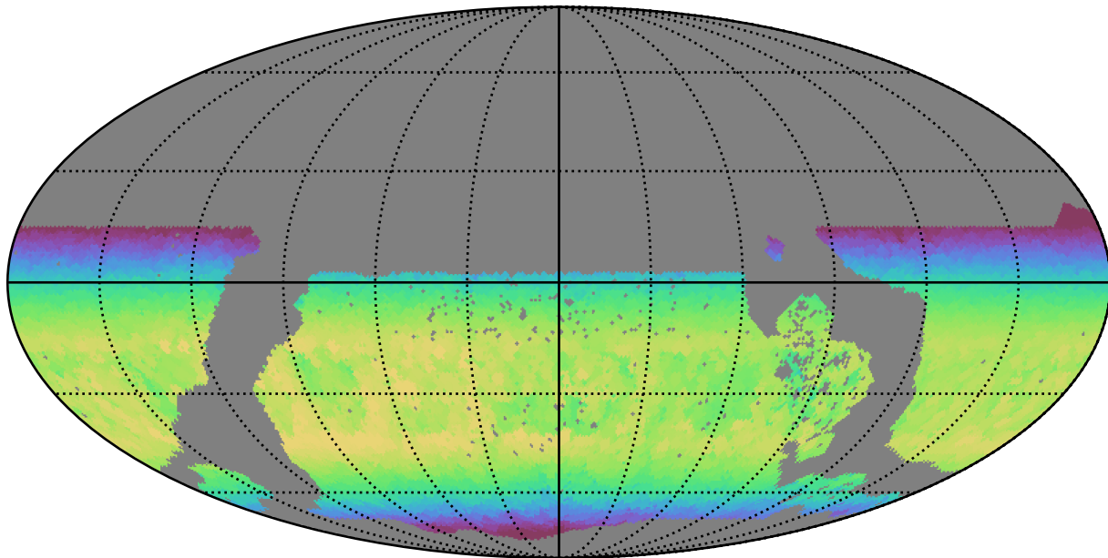
too_elab_r8_d2_giz_v3.4_10yrs WFD y band: Max skyBrightness
