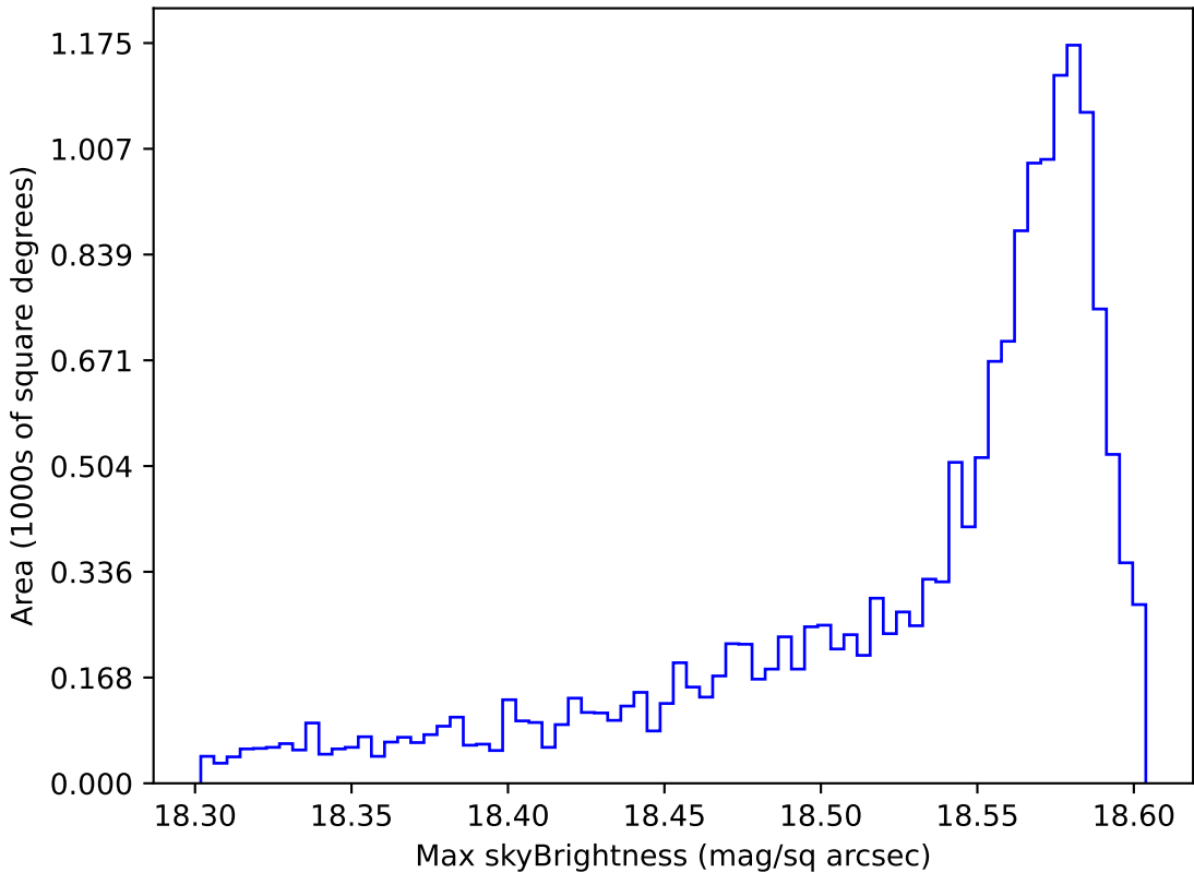
too_elab_r8_d2_giz_v3.4_10yrs WFD y band: Max skyBrightness
