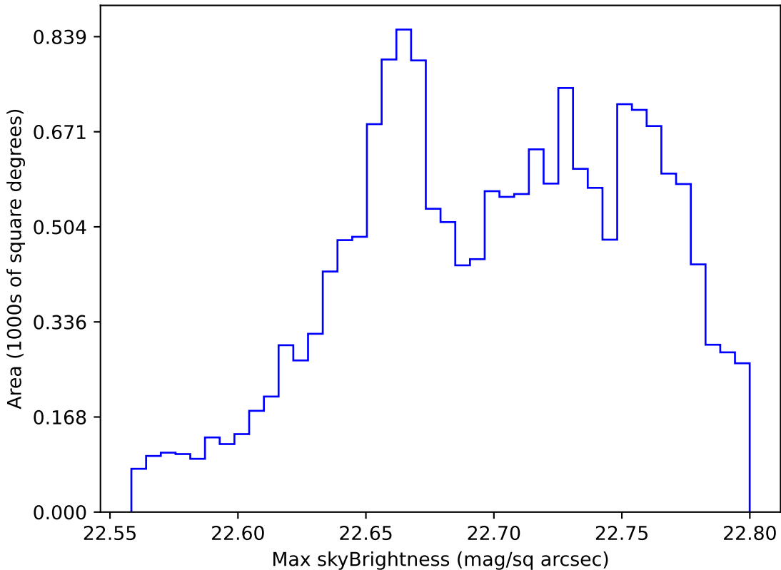
too_elab_r8_d2_giz_v3.4_10yrs WFD u band: Max skyBrightness
