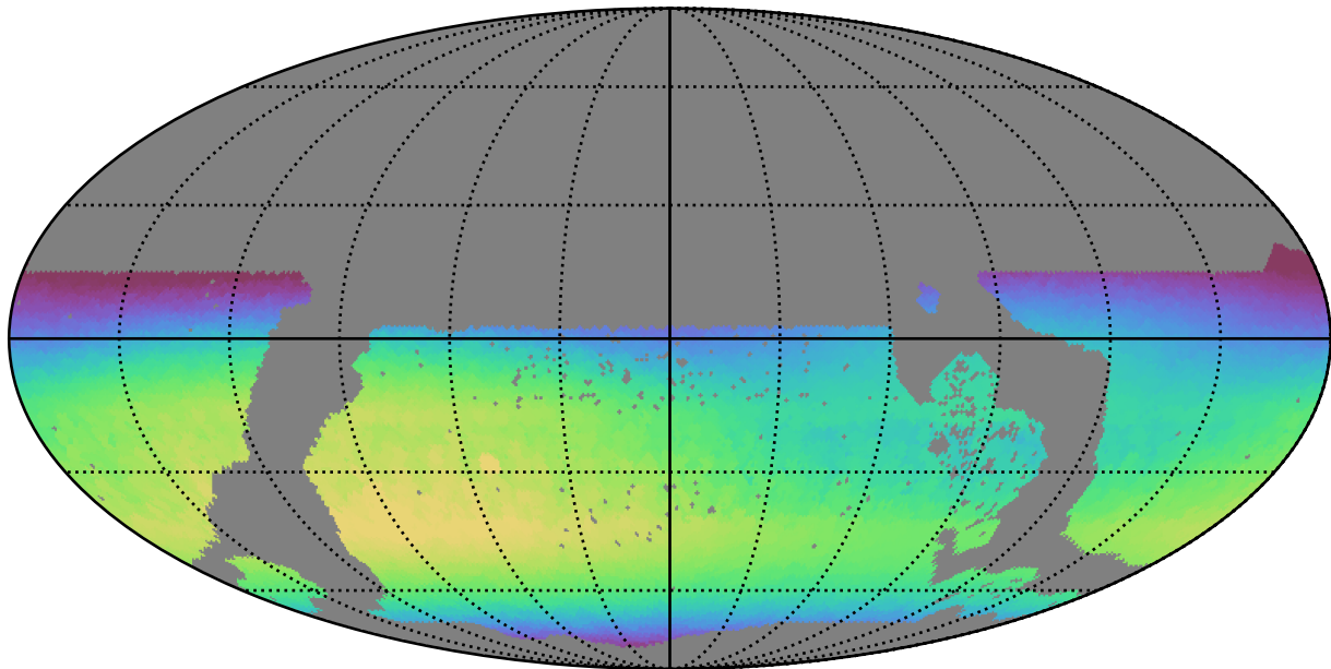
too_elab_r8_d2_giz_v3.4_10yrs WFD i band: Max skyBrightness
