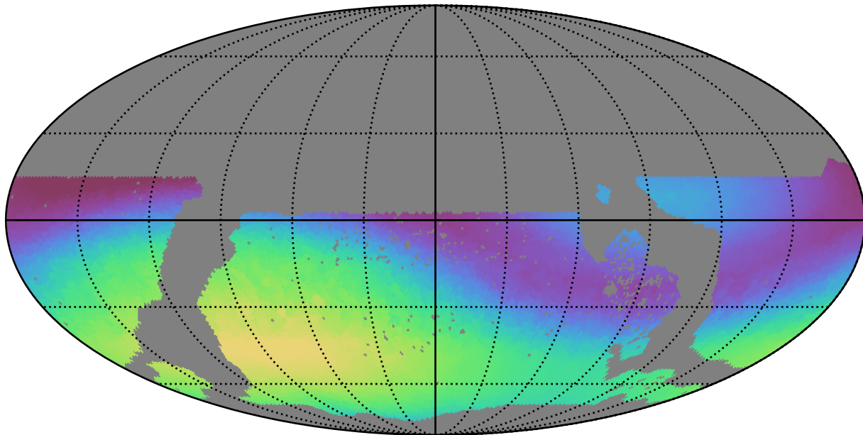
too_elab_r8_d2_giz_v3.4_10yrs WFD g band: Max skyBrightness
