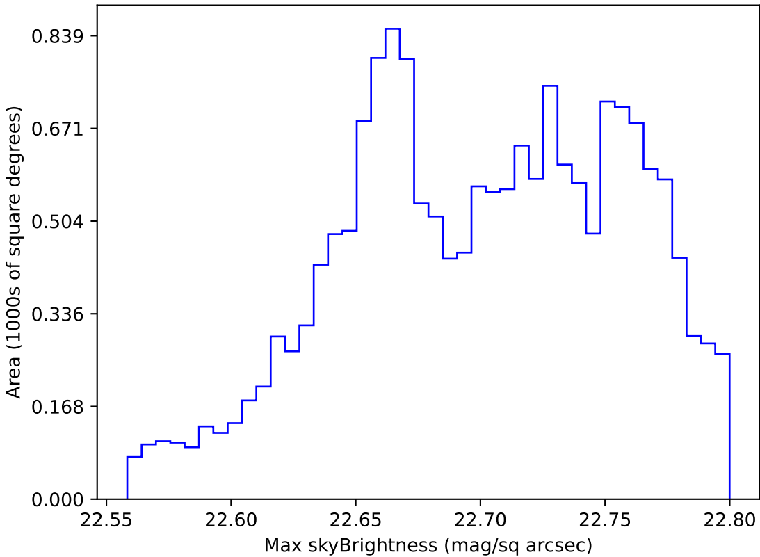
too_elab_r8_d2_giz_v3.4_10yrs WFD all bands: Max skyBrightness
