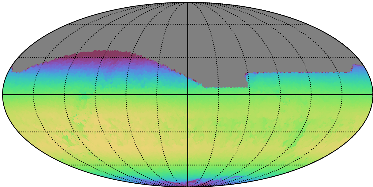
too_elab_r8_d2_giz_v3.4_10yrs All sky z band: Max skyBrightness
