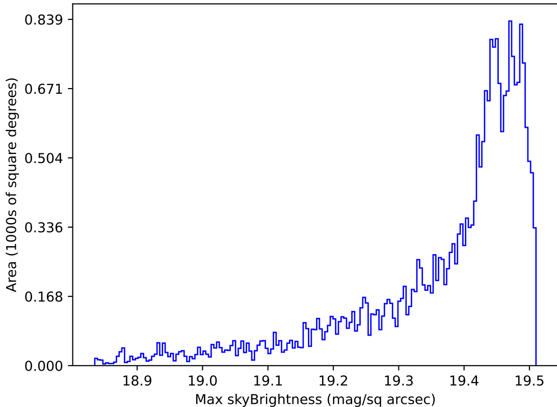
too_elab_r8_d2_giz_v3.4_10yrs All sky z band: Max skyBrightness
